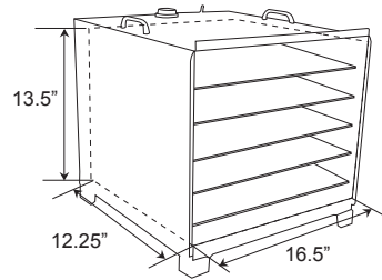
INNER DIMENSIONS
